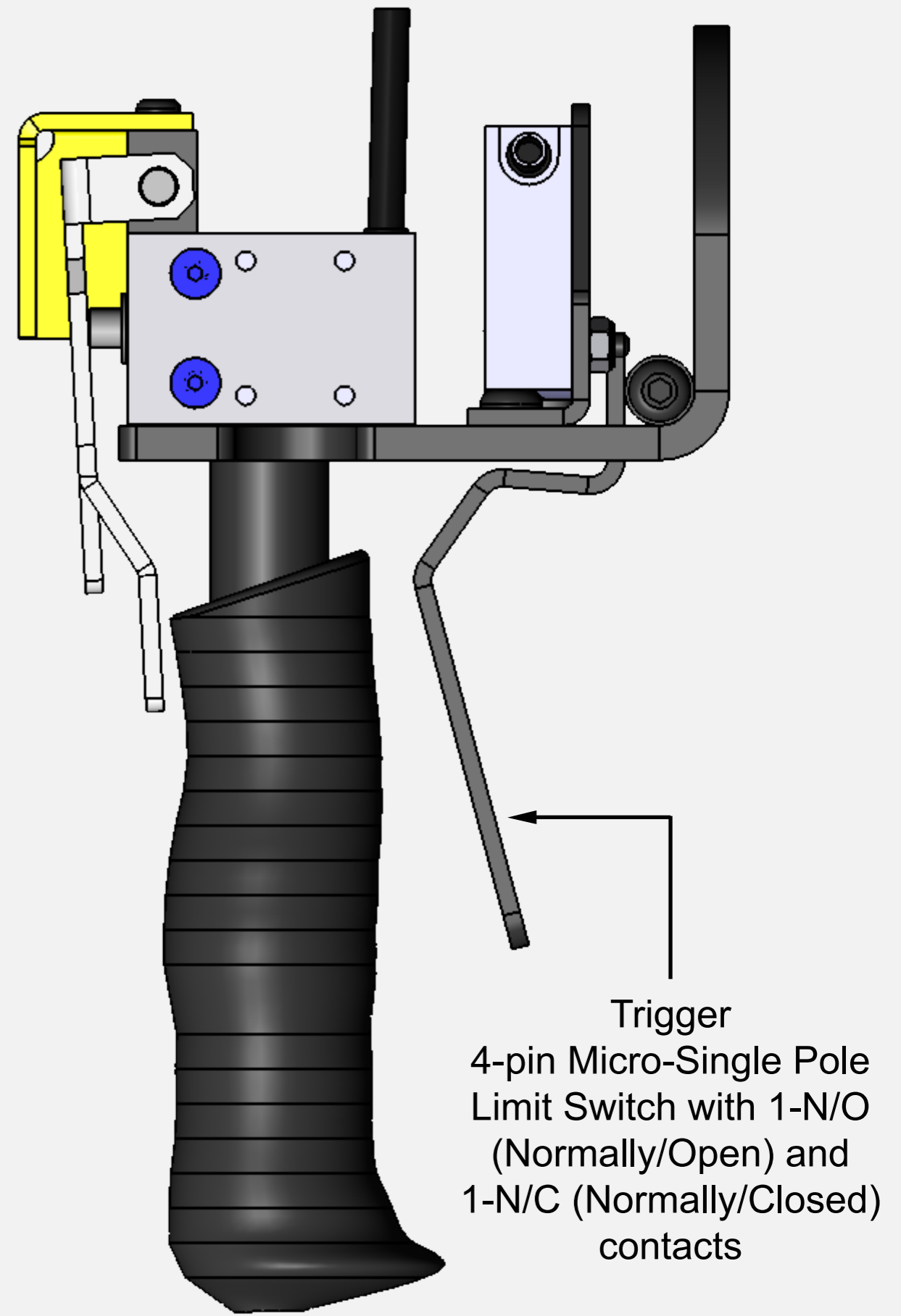
4-pin Micro-Single Pole Limit Switch with 1-N/O (Normally/Open) and 1-N/C (Normally/Closed) contacts.
