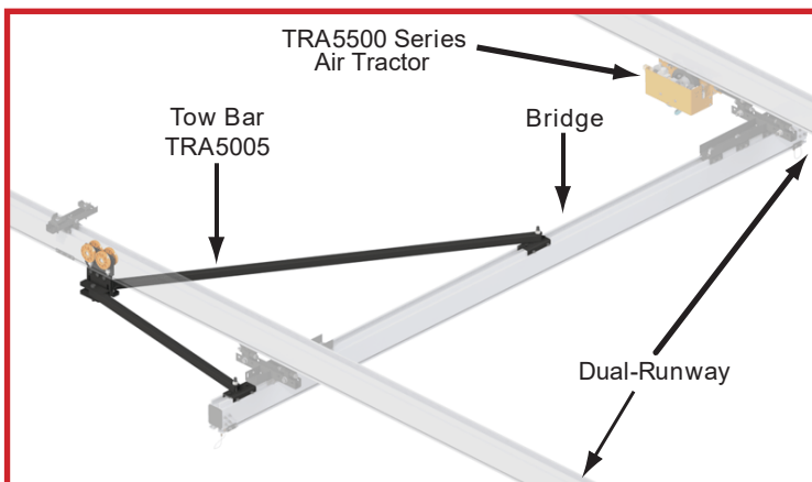
Dual-Runway Configuration
