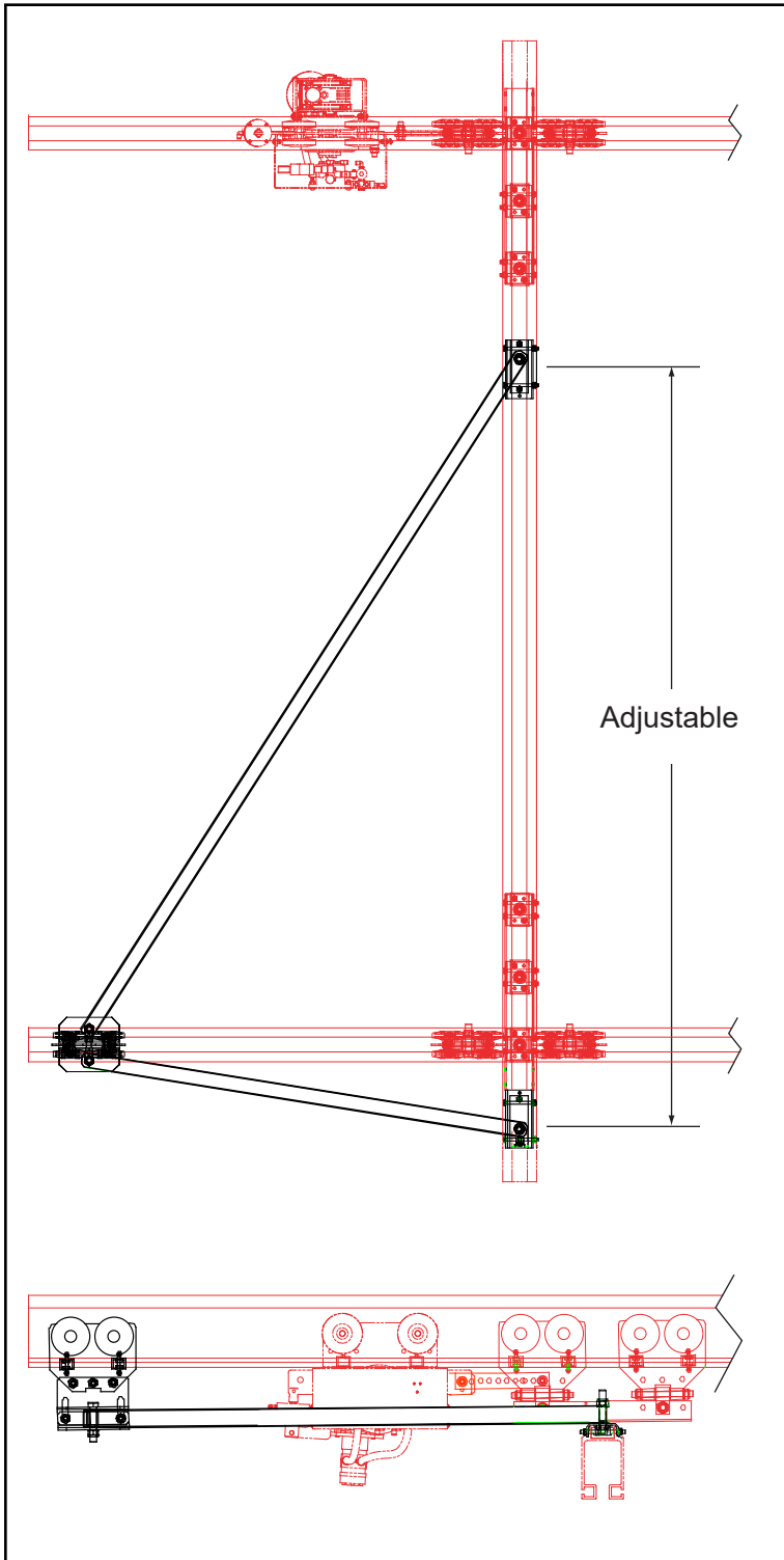
Dual Runway
