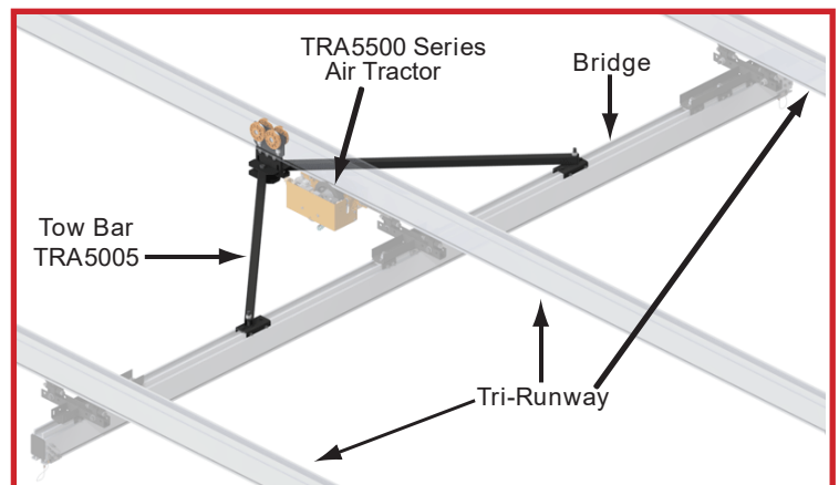
Tri-Runway Configuration
