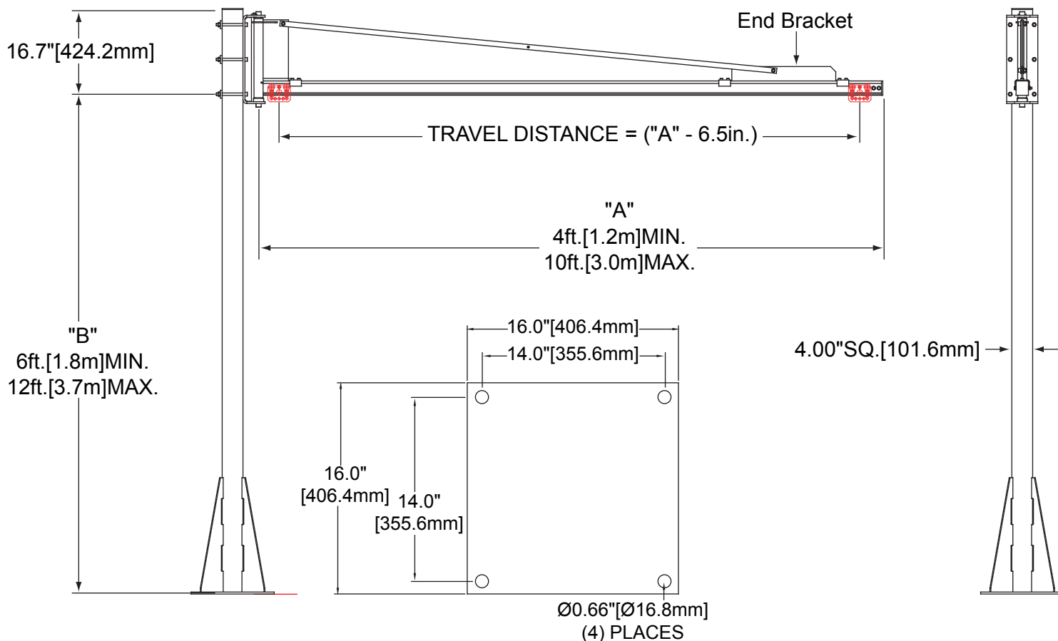
BASE PLATE HOLE PATTERN
